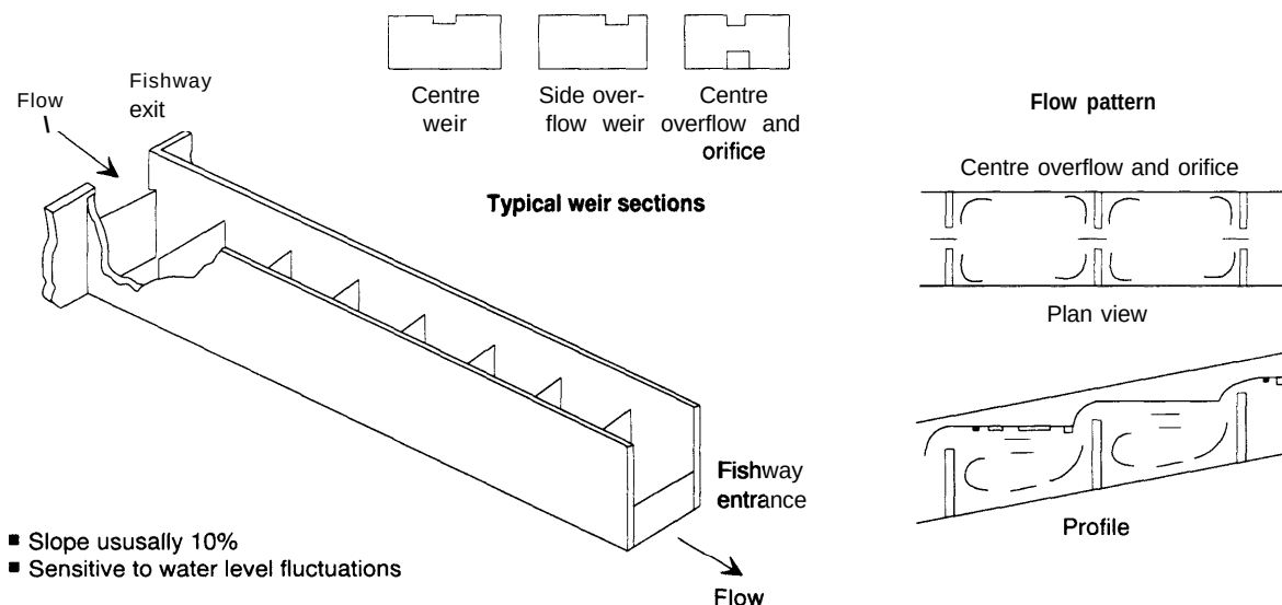
FIGURE 3-1: Weir Fishway
